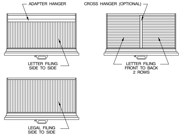
FIREKING 31" LATERAL FILING ARRANGEMENTS
