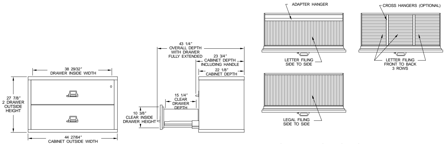
FIREKING 44" LATERAL FILING ARRANGEMENTS
